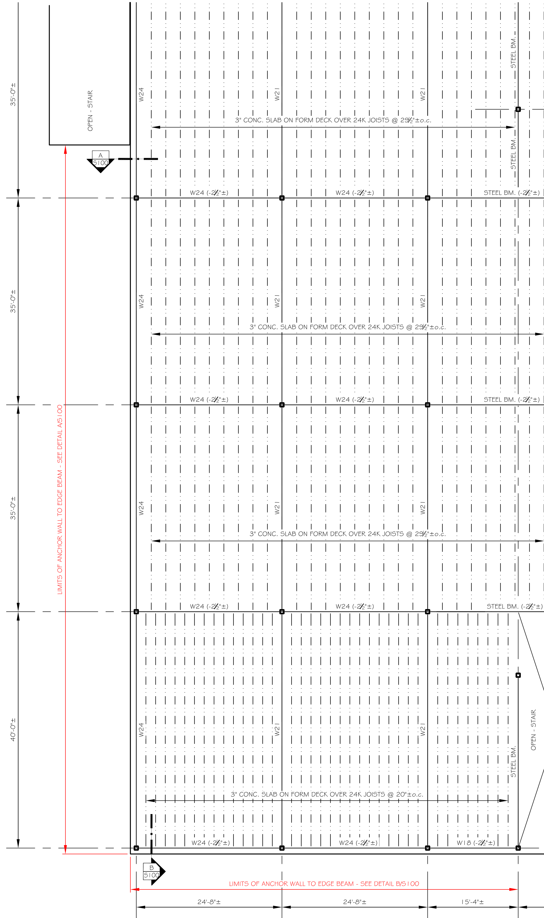
PARTIAL FLOOR FRAMING PLAN SCALE : 1/8" = 1'-0" NOTES: 1. SEE SHEET S100 FOR GENERAL STRUCTURAL NOTES. 2. ALL FRAMING SHOWN IS EXISTING UNLESS NOTED OTHERWISE.
